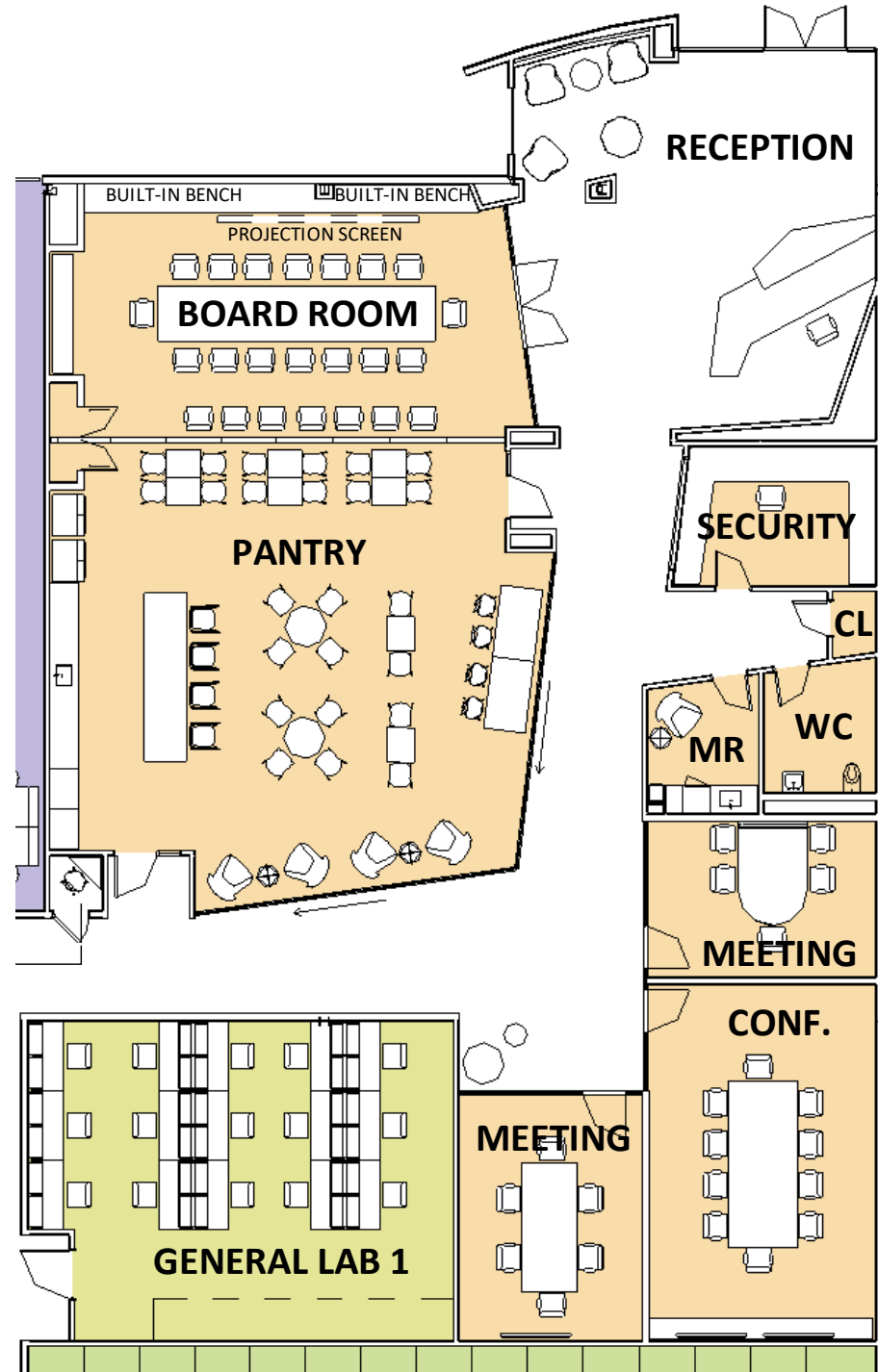
1 | GENERAL LAYOUT
